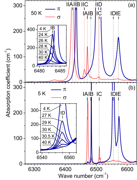
FIG. 10. (Color online) Emergent lines in the low-temperature spectrum of the ^3F_3 multiplet. The Insets show in detail the rise of the lines (a) IB and (b) ID below T_N .
